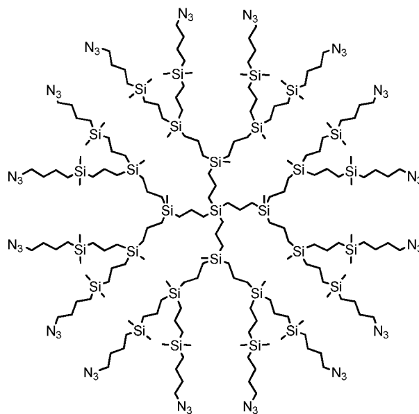
G_3-[Si-CH_2CH_2CH_2CH_2N_3]_{16} (32)
