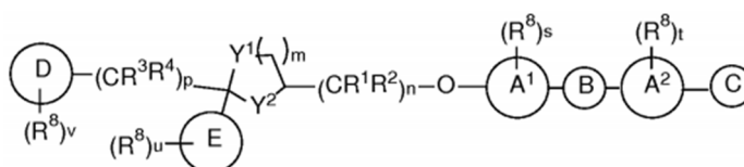
Formula (I)
