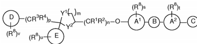
Formula (II)
