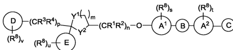
Formula (II)
