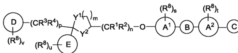
Formula (II)
