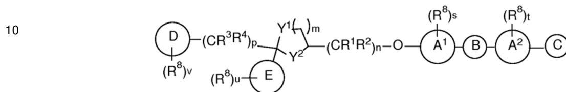
Formula (I)
