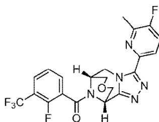
Ejemplo 160: (2-fluoro-3-(trifluorometilo)fenilo)(6R,10S)-3-(5-fluoro-6-metilpiridina-2-ilo)-6,7,9,10-tetrahidro-5H-6,10-epimino[1,2,4]triazolo[3,4-d][1,5]oxazocina-11-ilo)metanona.
