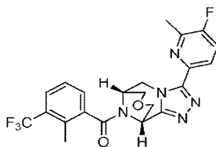
Ejemplo 160: (2-fluoro-3-(trifluorometilo)fenilo)(6R,10S)-3-(5-fluoro-6-metilpiridina-2-ilo)-6,7,9,10-tetrahidro-5H-6,10-epimino[1,2,4]triazolo[3,4-d][1,5]oxazocina-11-ilo)metanona.
